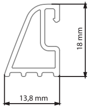
AURA KY - X1 EASY ENTRY
