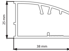
X1 - X0 - CLASSICS PS X1 EASY ENTRY Yan Panel Dönüş Profili
