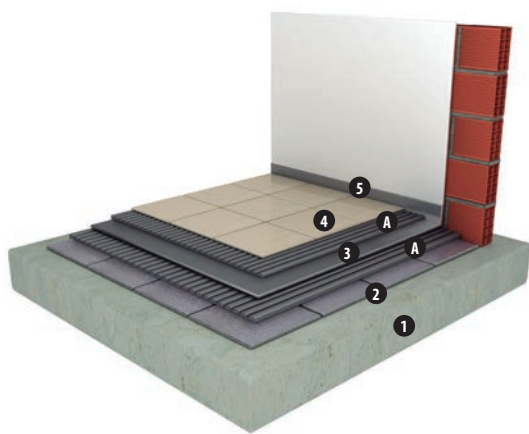
1- floor slab 2- old floor tile 3- fonopac R 4- floor tile 5- bandin A- cement-based adhesive + fonolax
