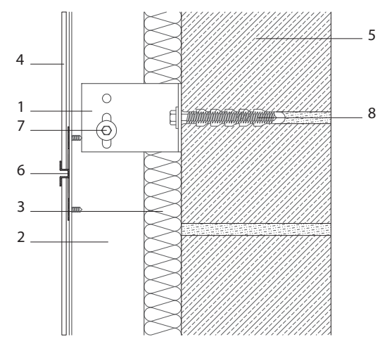
Vertical section
