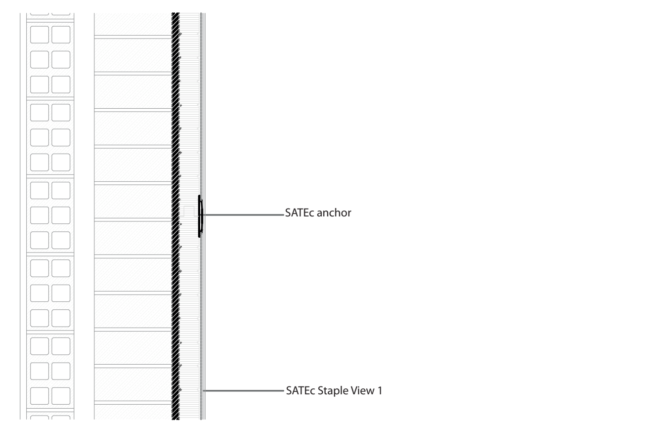
SATEc Air Slate system. Vertical section Wall
