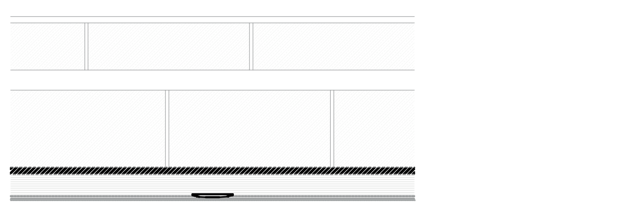
SATEc Air Slate system. Horizontal section. Wall
