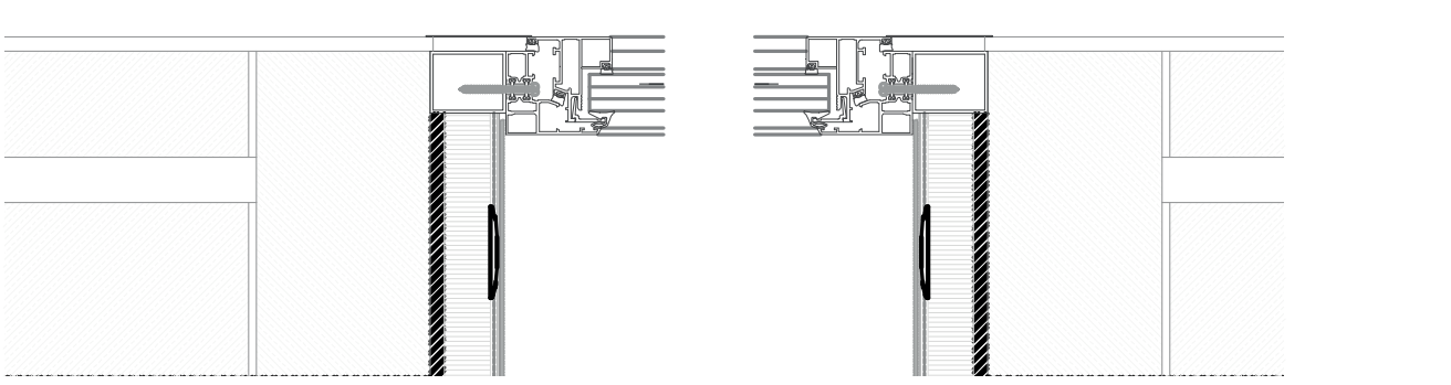
SATEc Air Slate system. Horizontal section. Gap / space
