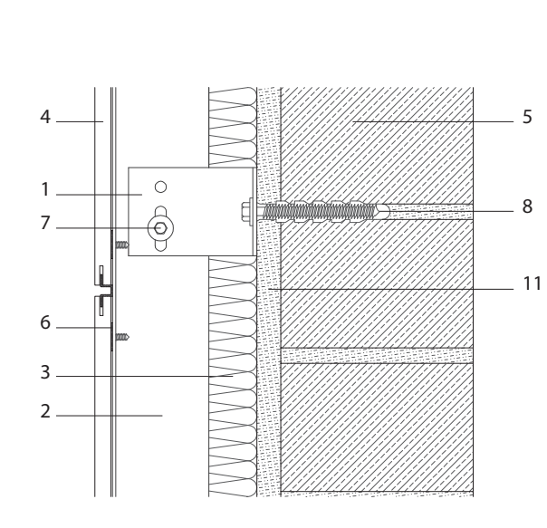
Vertical section
