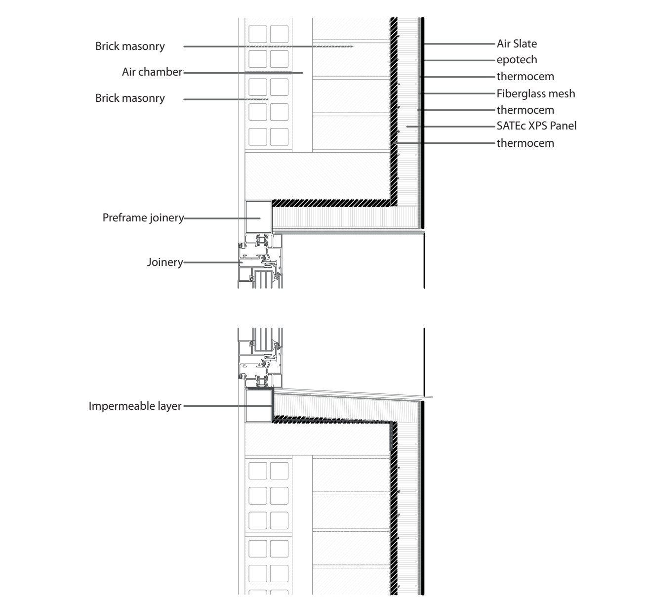
SATEc Air Slate system. Vertical section Gap / space
