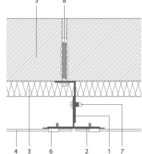
Horizontal section
