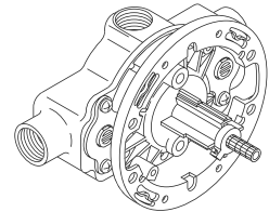
Pressure-Balancing Valve
