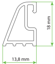
AURA KY - X1 EASY ENTRY
