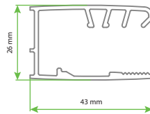
SOLVA - DESIGN PURE SAK YP Donus Profili
