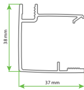
X1 - X0 - CLASSICS PS X1 EASY ENTRY Yan Panel Dönüş Profili
